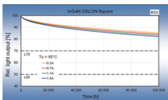
Lifetime curve
