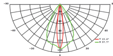
Distribution Curve
