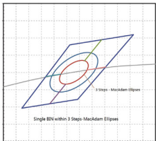
MacAdam Ellipses
